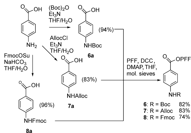
Scheme 2. Synthesis of the orthogonally protected legs.
