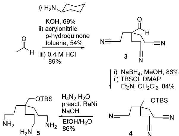
Scheme 1. Synthesis of the core.
