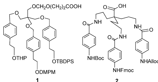
Figure 1. Structure of previously developed scaffold 1 and structure of the new tripodal scaffold 2 .
