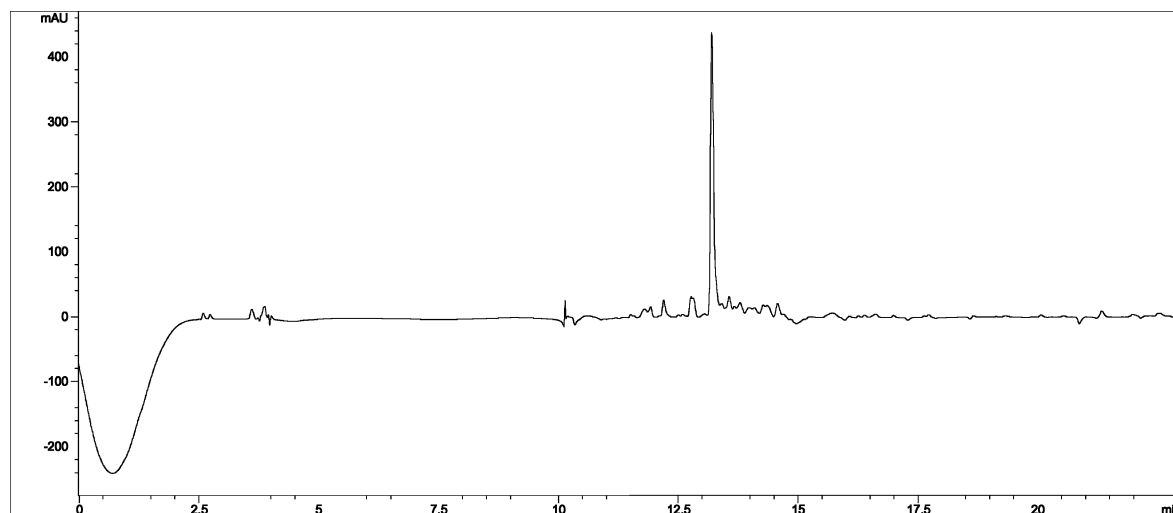
Figure 3. LC at 214 nm of the crude tripodal peptide obtained after photolysis of 12 .
