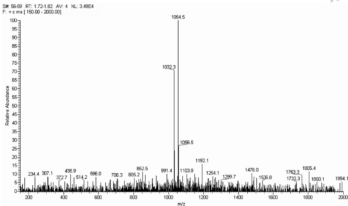
Figure 4. ES-MS + of the crude tripodal peptide obtained after photolysis of 12 .
