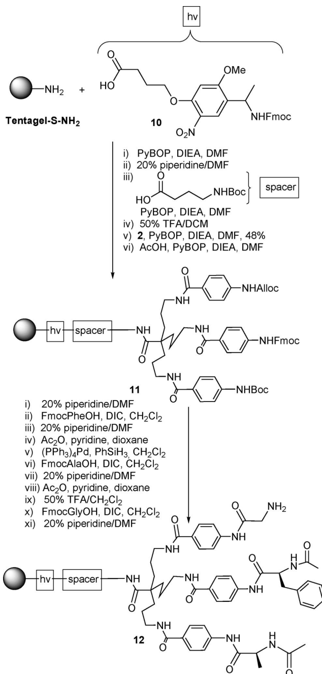
Scheme 4. Solid-phase synthesis of a possible library member.
