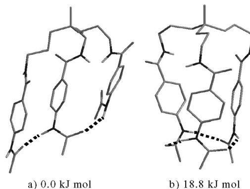
Figure 2. Results of molecular modelling studies on a simplified version of 2 . [5] Two energetically favoured conformations in H 2 O are shown. The dotted lines represent intramolecular H-bonding.
