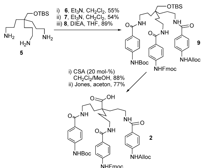
Scheme 3. Assembly of scaffold 2 .
